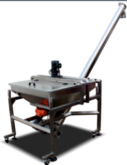
SCREW FEEDER
